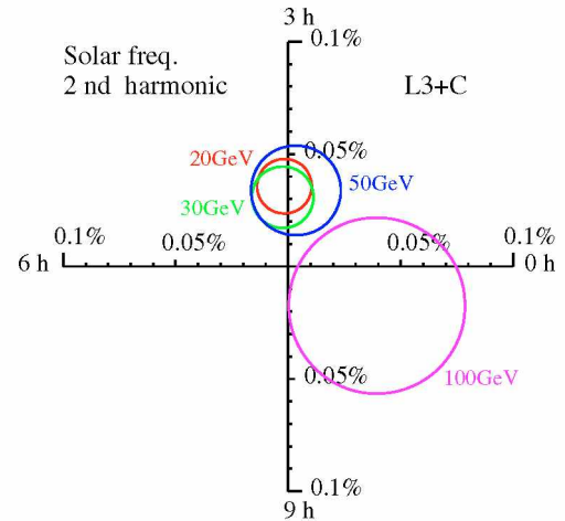
Fig. 11. Dial plots showing the amplitude and the phase of the second harmonic of the anisotropy function at the Solar frequency for four different muon energy-cuts. The circles represent the 68.5% confidence level region.
